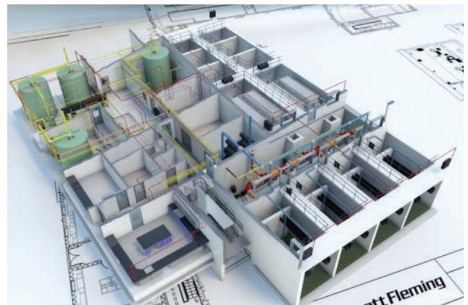
BIM perspective of the Red Lion Municipal Authority Cabin Creek Water Treatment Plant, Pa.
